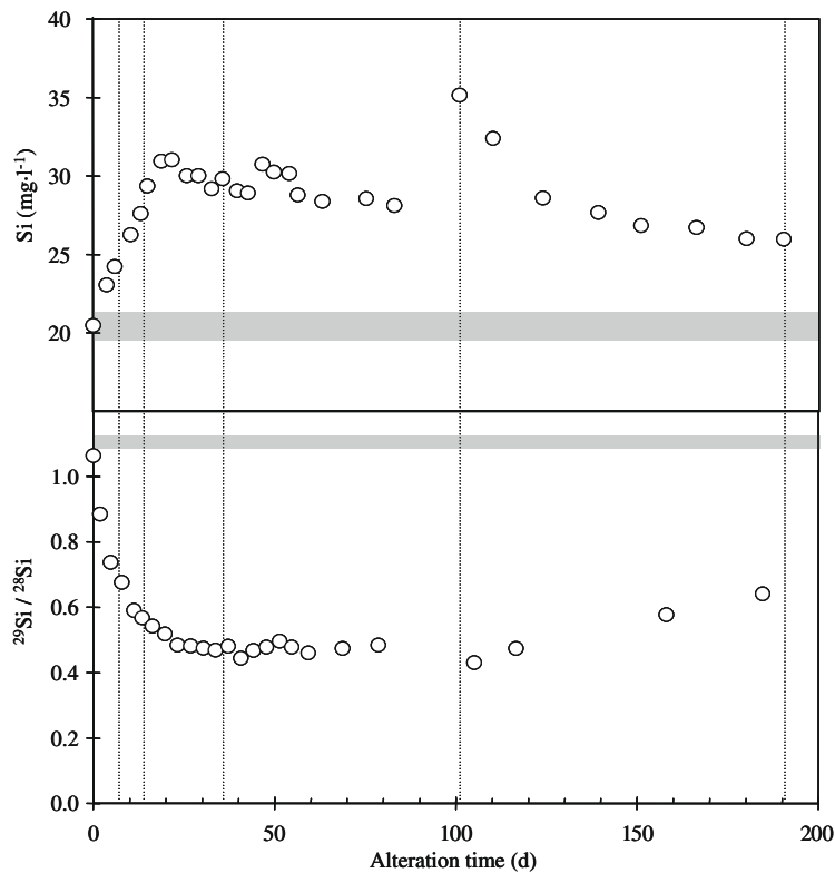
Fig. 12. Evolution of silicon concentration and isotopic ratio 29 Si/ 28 Si in the leachate with time of alteration. The isotopic analyses have a precision better than 1% whereas elemental analyses of silicon have a precision of 5%. Grey horizontal lines correspond to the initial silicon concentration and isotopic ratio of the solution, respectively.
