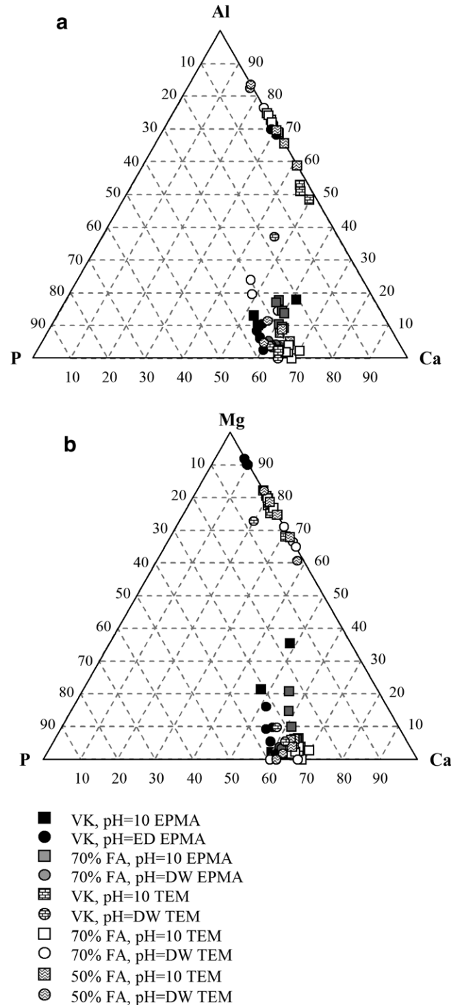
Fig. 7. Ternary diagram in atomic proportion of (a) Al, Ca and P, and (b) Mg, Ca and P. EMPA and TEM analyses performed on VK, 50% and 70% FA altered at pH = DW and 10, 80 °C and during 181 days.
