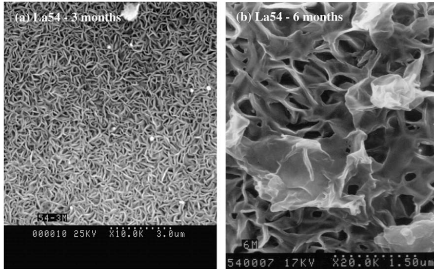
Fig. 4. SEM microphotographs (secondary electrons) of altered glass surface after (a) 3 months and (b) 6 months. Phyllosilicates recovered the surface.
