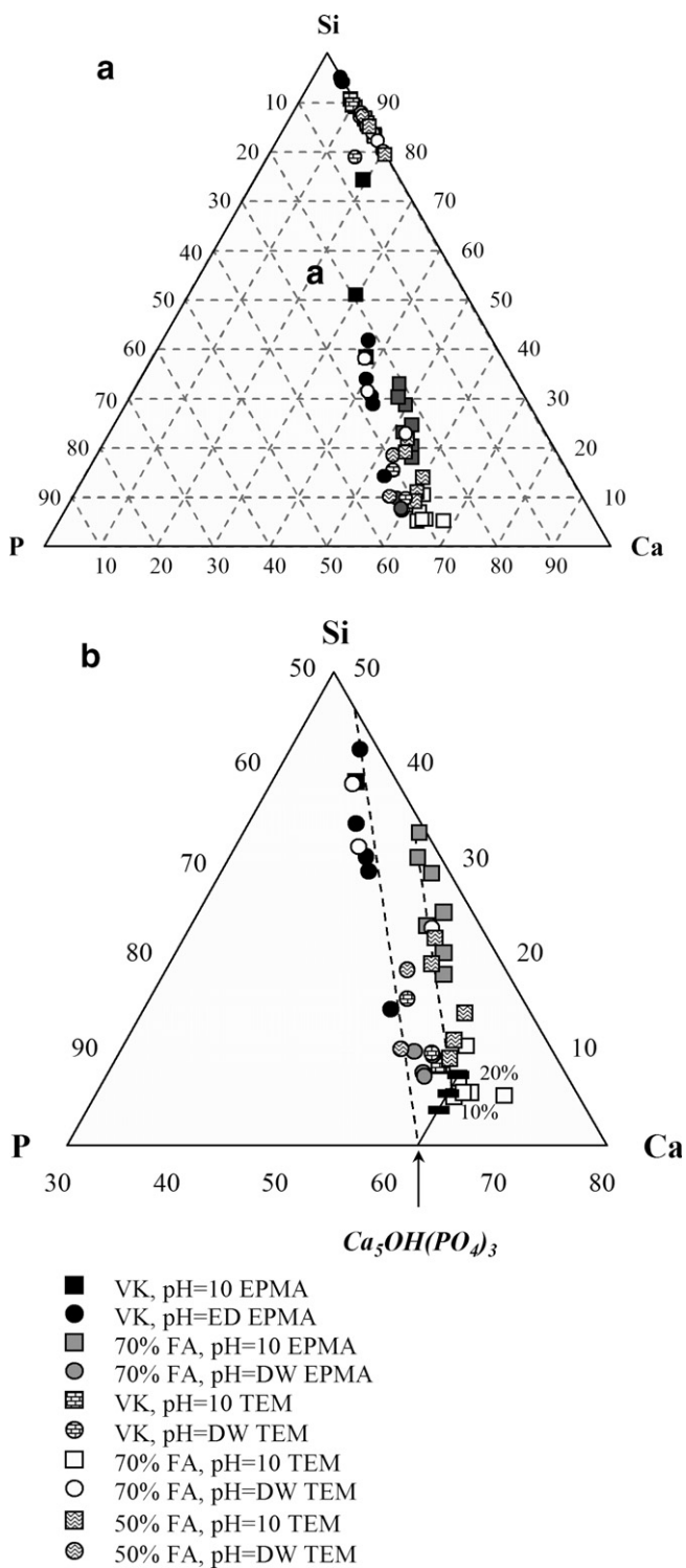
Fig. 6. (a) Ternary diagram in atomic proportion of Si, Ca and P. EMPA and TEM analyses performed on VK, 50% FA and 70% FA glasses altered at pH = DW and 10, 80 °C and during 181 days. (b) Detail of (a) for Si(50%)–P(30–80%). The stoichiometry of hydroxyapatite is plotted with different Si–P substitution ratio (10%, 15%, 20%, black rectangles).
