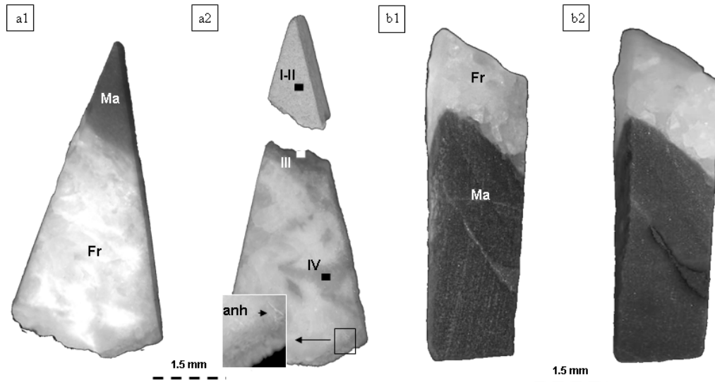
Figure 1: Observation with binocular lens of the rock samples before and after experiment. (a1) and (b1) samples before experiment, (a2) sample after experiment with the gas mixture, (b2) sample after experiment with pure CO 2 . (anh) glitter of anhydrite, (Ma) Matrix of the rock, (Fr) fracture of the rock. Points I to IV refer to pictures on Figure 3.
