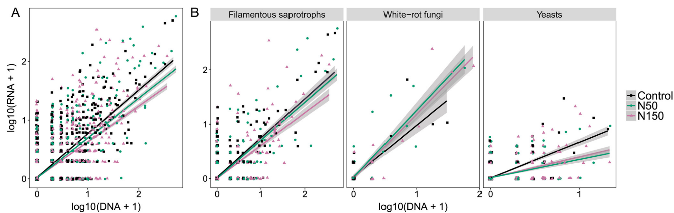
Fig. 3. Fungal activity among N treatments for (A) the whole fungal community and (B) decomposer functional groups. Points represent the sequence abundance of individual OTUs and lines represent the relationship between total (DNA) and active (RNA) community OTUs in each treatment as estimated by linear regression, with the gray band representing the 95% confidence interval as estimated by the R package ggplot2 (Wickham, 2009). Overplotting of points was avoided by allowing the points to move 0.015 units along the x- or y-axis using the position_jitter function in ggplot2.
