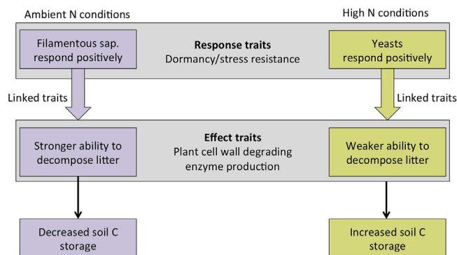
Fig. 5. Conceptual understanding of fungal responses to soil N enrichment and feedbacks to soil C storage (adapted from Treseder and Lennon, 2015).
