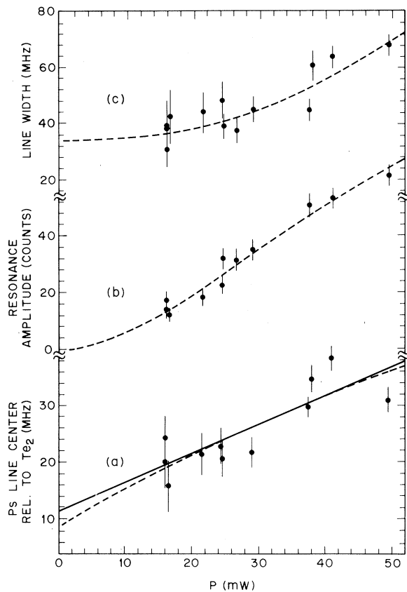
FIG. 3. Frequency shift, linewidth, and resonance amplitude plotted vs transmitted laser power. The simultaneous fit of three theoretical curves to the data is given by the dashed lines. The simple quadratic Stark shift is shown by the solid line and is listed in Table I.
