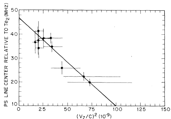
FIG. 2. Ps line center relative to the \text{Te}_2 reference line plotted vs v_z^2/c^2 showing the second-order Doppler shift. The straight line intercepts the v_z^2 = 0 axis at 46.7 \pm 3.3 MHz with \chi^2/\nu = 8.13/8 .
