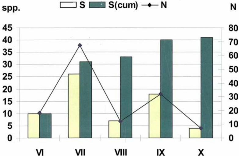
Fig. 10: Phenology of early rove beetle (Staphylinidae) succession on a restored gravel bank on the River Adige (Lana, Italy) in 2003. (S: species number, S(cum): cumulative species number, N: individuals captured).
