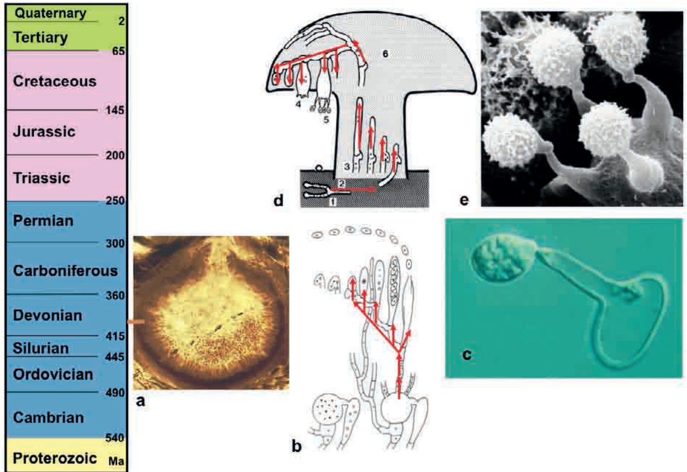
Fig. 4: The dikaryomycotic fungi, Ascomycota and Basidiomycota. a: Fossils of Ascomycota are known from the Devonian. The perithecium is approximately 400 μm in diameter and develops in the stomatal chamber of Asteroxylon . Their morphology is identical with extant representatives. The dikaryophases of typical Asco- and Basidiomycota are illustrated schematically (red arrows). b: In Ascomycetes the dikaryophase is restricted to short hyphae between the ascogon and the asci. d: In the majority of Basidiomycetes the dikaryophase extends to more or less the whole life cycle. e: Ballistospores ejected from sterigmata are typical for basidiomycetous meiosporangia, the basidia. c: A similar mechanism can occur in ballistosporous yeasts of Basidiomycetes. a from TAYLOR et al. (1999). Orig. F. OBERWINKLER.
